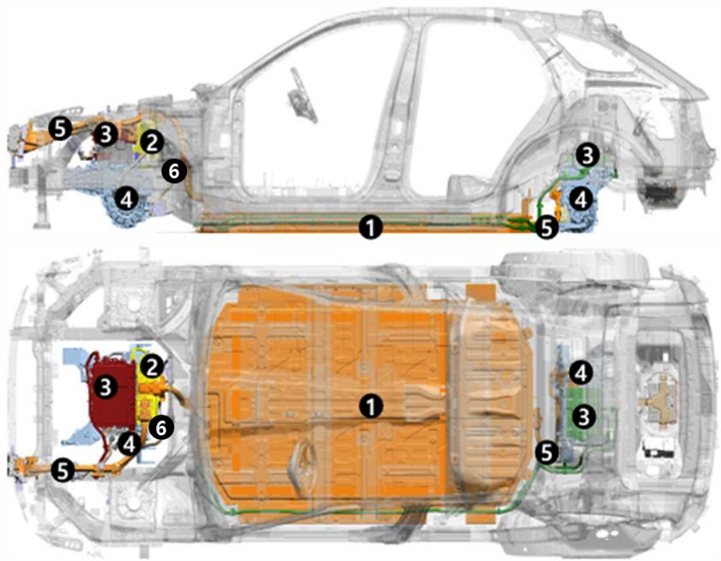
Location of High-Voltage Components
