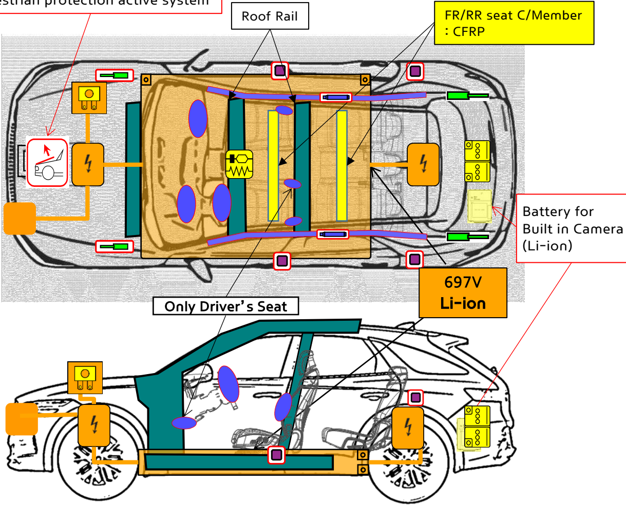
Pedestrian protection active system
